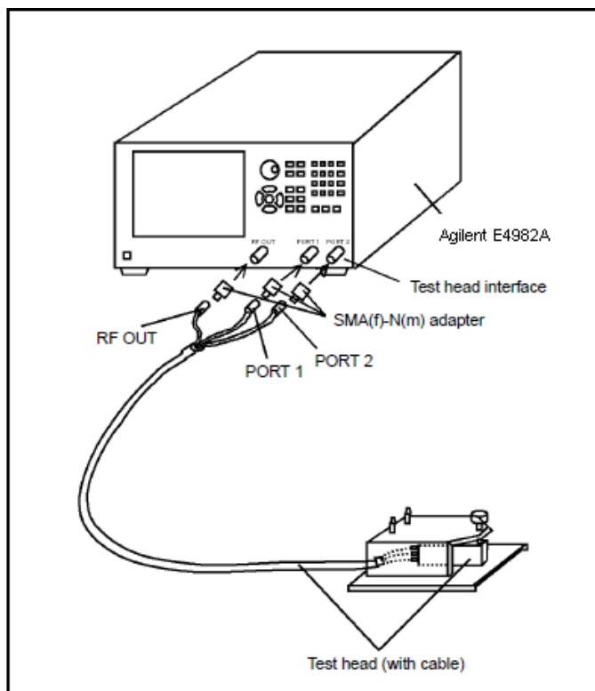
Figure 5 Connecting test head cable to E4982A
